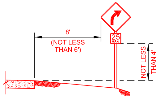
WARNING SIGN WITH ADVISORY SPEED PLATE NON-URBAN DISTRICT
