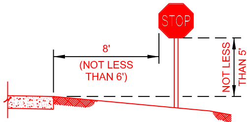
ROADSIDE SIGN NON-URBAN DISTRICT
