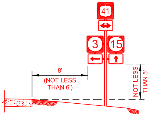
ROADSIDE ASSEMBLY NON-URBAN DISTRICT
