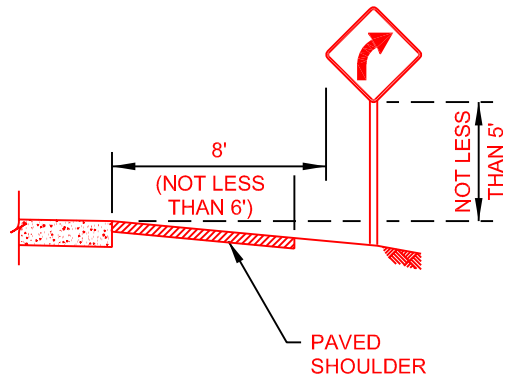
ROADSIDE SIGN NON-URBAN DISTRICT
