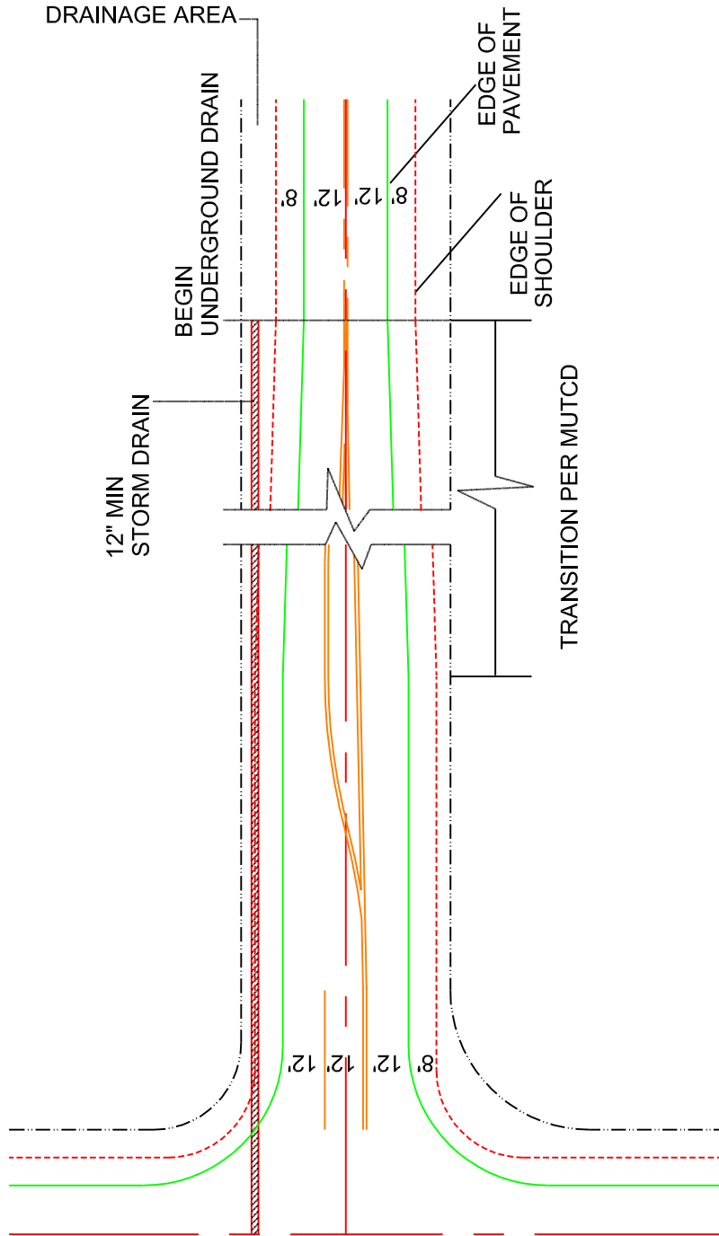
NOTE : TYPICAL UNDERGROUND DRAIN
