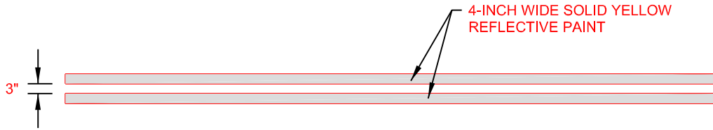
TYPE 1 CENTERLINE
