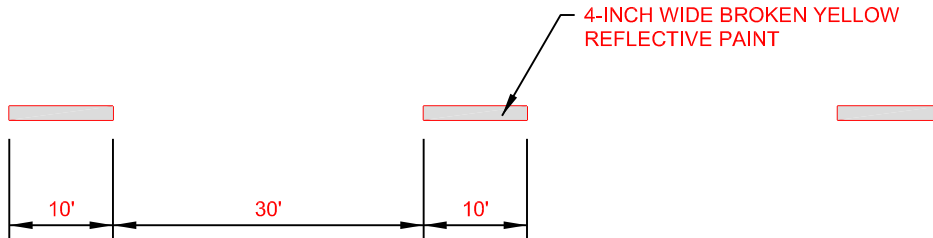
TYPE 3 CENTERLINE
