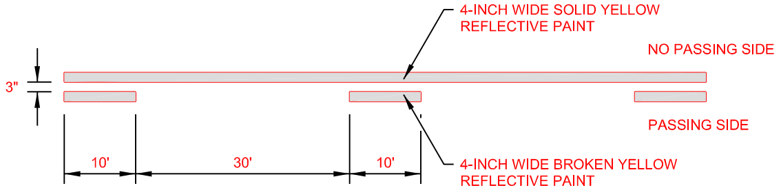
TYPE 2 CENTERLINE
